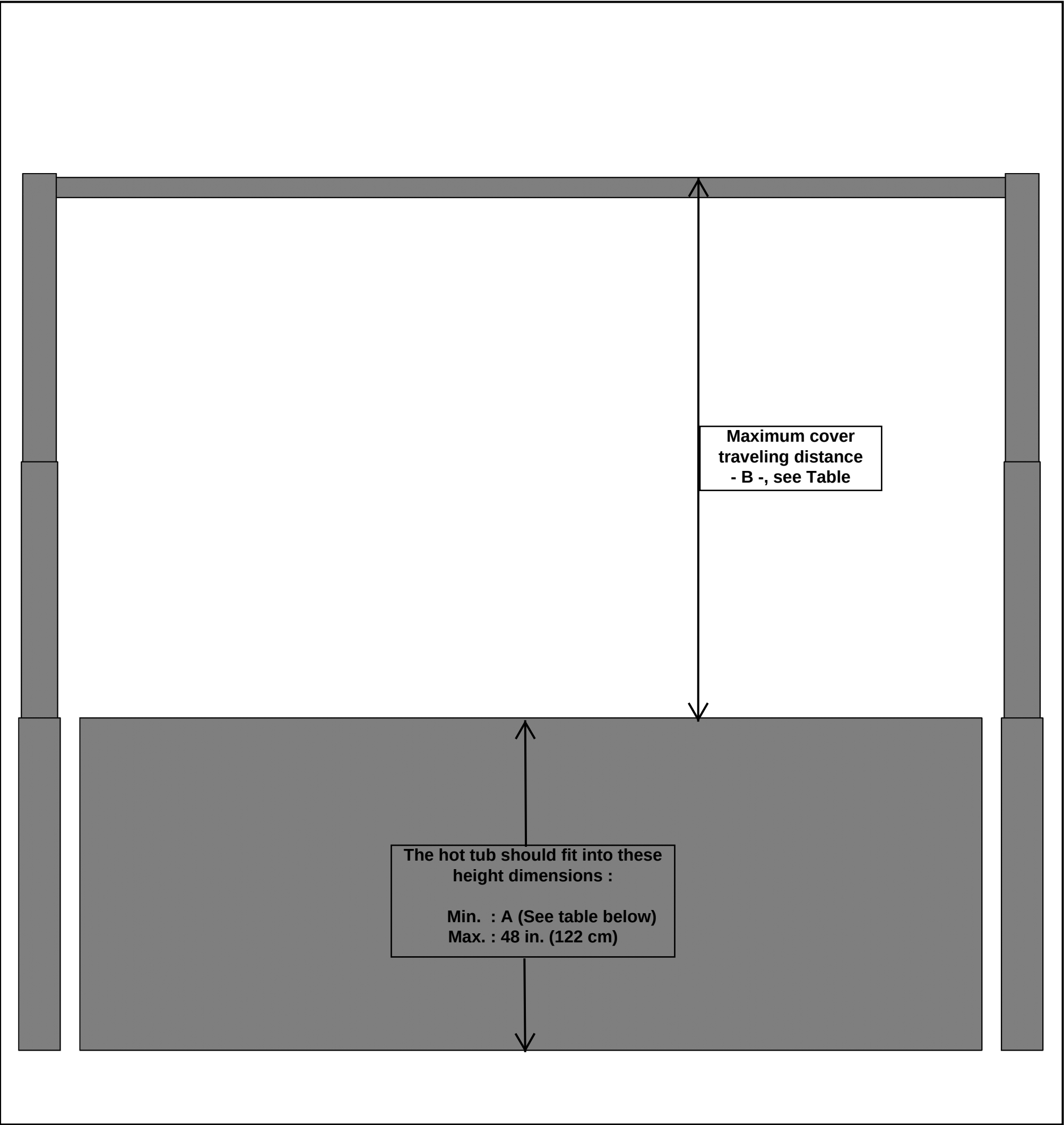
Covana Evolution - Side Elevation Dimensions
